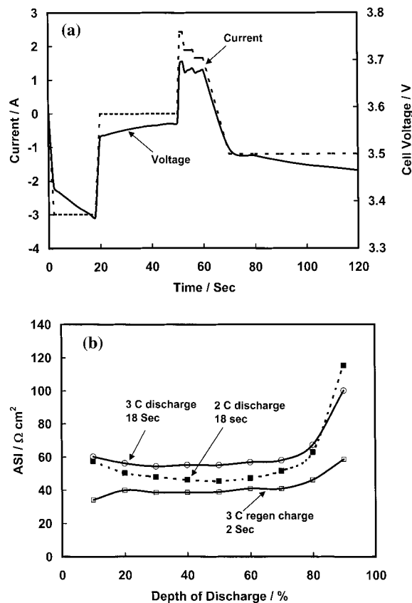
Fig. 4. 18650 cell: (a) Voltage response to HPPC profile shown in Figure 1; (b) \text{ASI}_t as function of DOD to HPPC profile containing \text{LiNi}_{0.8}\text{Co}_{0.2}\text{O}_2 cathode.
